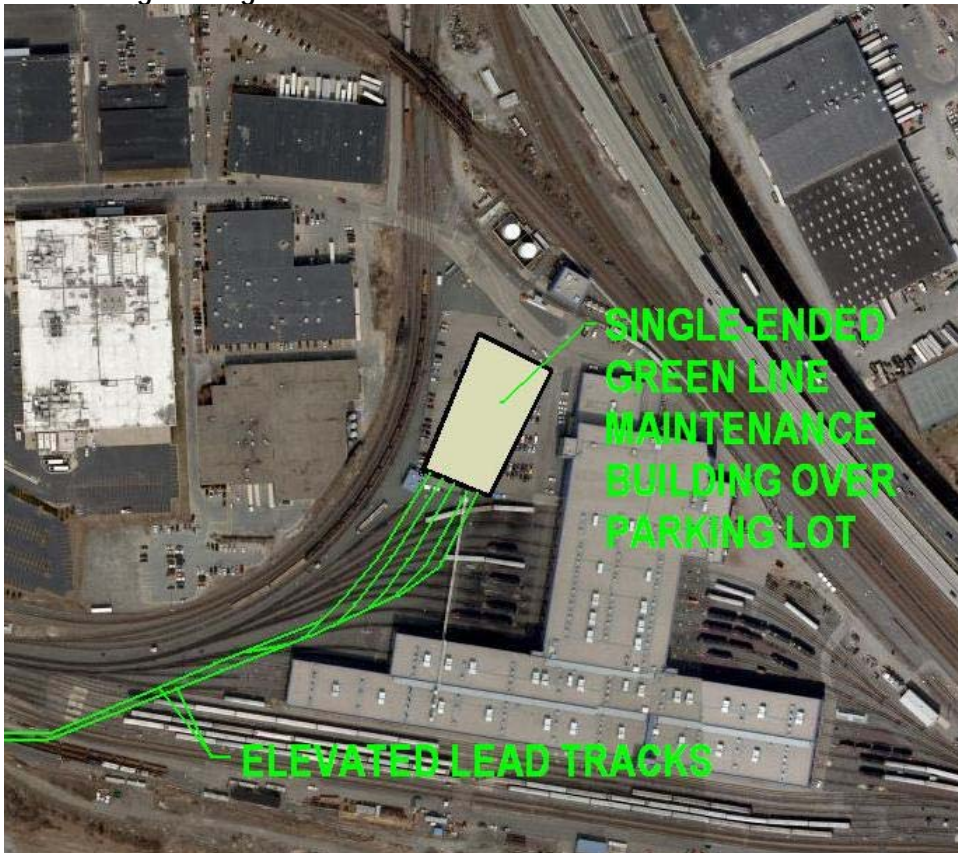
Figure 4: Layout of a Single-Ended Green Line Maintenance Building over the Existing Parking Lot
