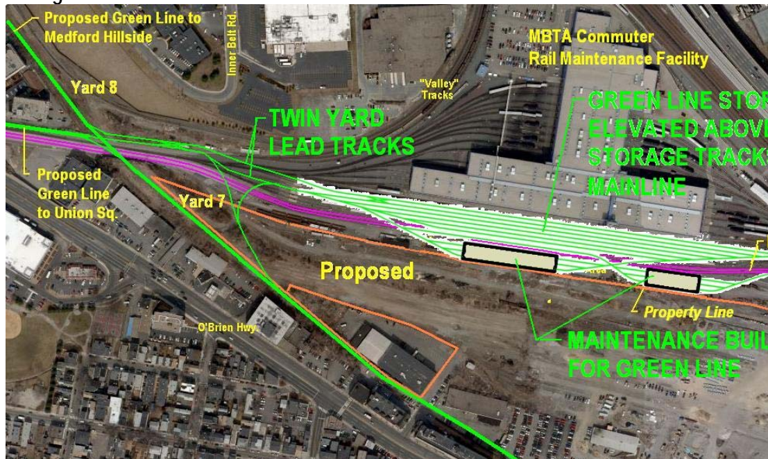
Figure 2: Elevated Green Line Storage/Support Facility over Existing Commuter Rail Storage Tracks
